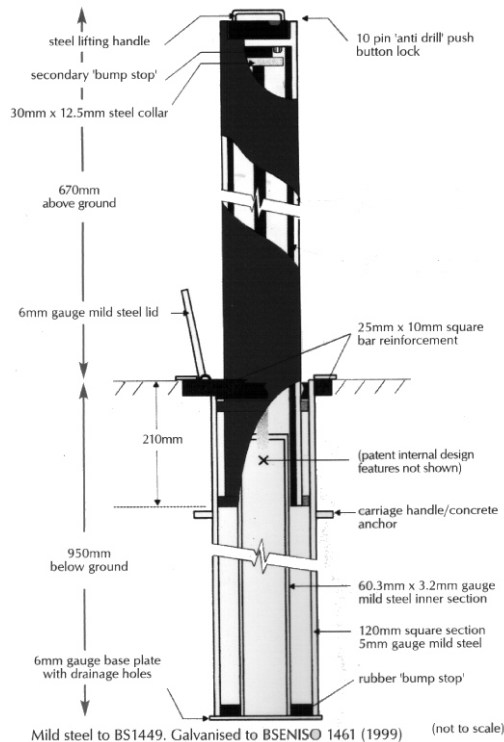
Telescopic Posts can be supplied with recessed reflective bands
